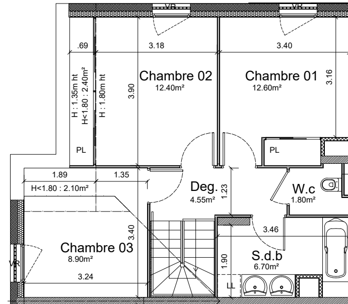
DUPLEX 46.95 m 2
